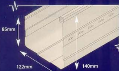
Stramit® M-Pattern Gutter Slotted
