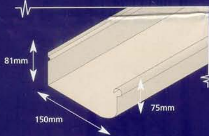
Stramit® Quad 150 Gutter Plain only
