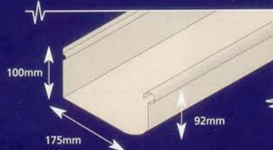
Stramit® Quad 175 Gutter Plain only
